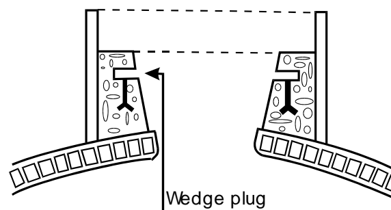
Figure 5.18 Position of the wedge plug
