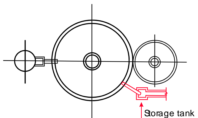
Figure 5.6 Slurry box drainage
